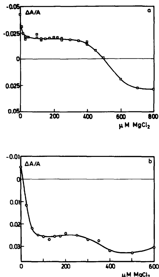
Fig.2. Reduced electric dichroism (at 6 kV/cm and 260 nm) of CE chromatin as a function of \text{MgCl}_2 concentration without (a) and with (b) spermine + spermidine in the preparation media.
