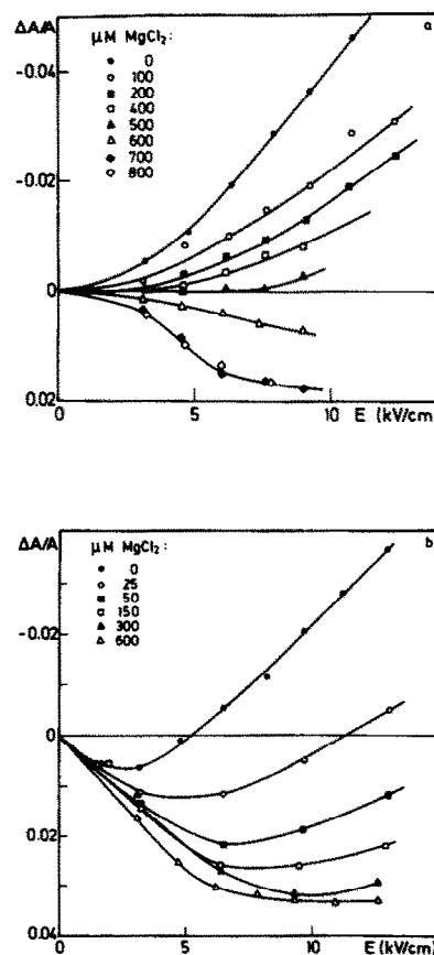
Fig.1. Field strength dependence of the reduced electric dichroism of CE chromatin at 260 nm for increasing \text{MgCl}_2 concentrations in 1 mM cacodylate buffer, pH 6.5, without (a) and with (b) spermine + spermidine in the preparation media.
