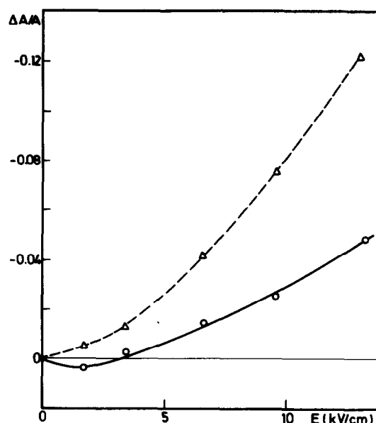
Fig.3. Field strength dependence of the reduced electric dichroism of CE chromatin at 260 nm. ( \circ ) Chromatin with spermine + spermidine in the preparation media; ( \Delta ) same sample as ( \circ ) dialyzed first against 1 mM cacodylate buffer, pH 6.5, with 0.5 M NaCl, then against the same buffer without NaCl added.
